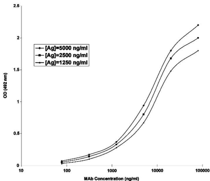
Figure 3. Experimental dose-response curve for anti hlgG monoclonal antibody 5F19G11 at three different h-IgG concentrations
