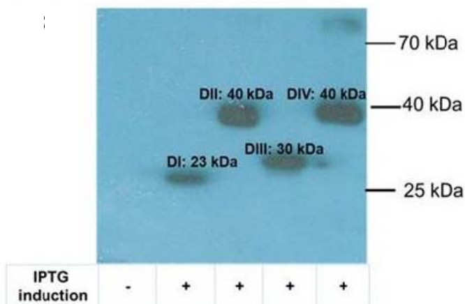
Figure 2. Detection of recombinant HER2 extracellular subdomains with anti-His tag antibody by immunoblotting. DI- pET-22b (+) and DIII- pET-22b (+) were transformed and expressed in BL21-DE3, whereas DII- pET-32a (+) and DIV- pET-32a (+) were expressed in RosettaGami.
