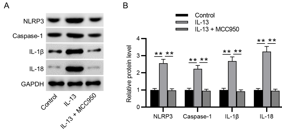
Supplementary Fig. 1. MCC950 inhibits NLRP3 inflammasome pathway in IL-13-treated hNECs. (A-B) Western blotting analysis of the protein levels of NLRP3, caspase-1, L-1β, and IL-18 in hNECs treated with IL-13 or/and MCC950. ^{**}p < 0.01 . NLRP3, NOD-like receptor family pyrin domain containing 3; IL-1β, interleukin-1β; IL-18, interleukin-18; hNECs, human nasal epithelial cells.
